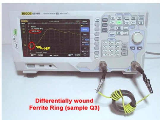
This differentially wound ring cancels out potentially high voltages and stray capacitance, while still providing excellent (-20dB) attenuation at HF frequencies
